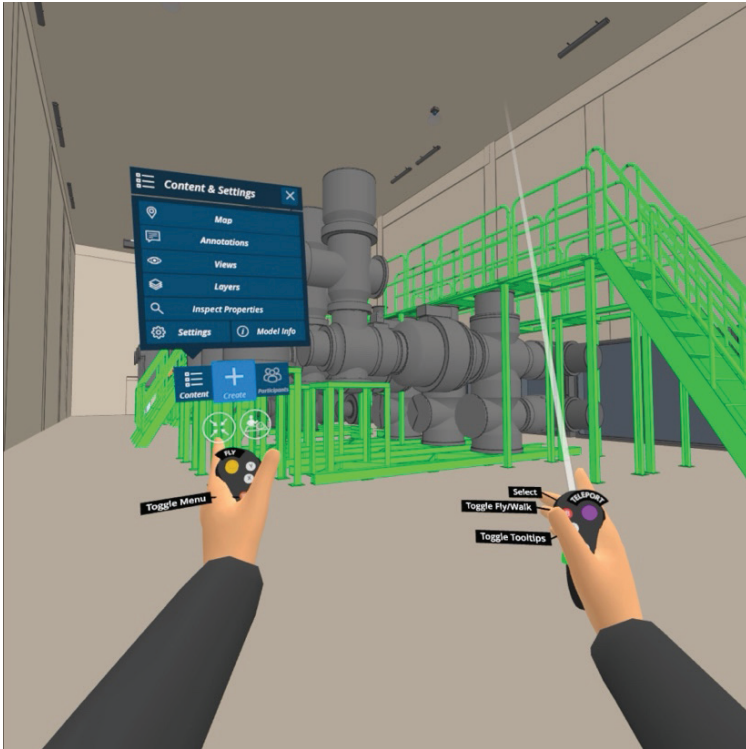
Figure 1. AutodeskXR’s interface.
