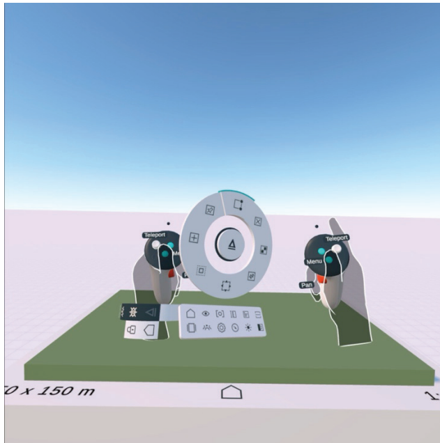
Figure 4. Arkio's interface.
